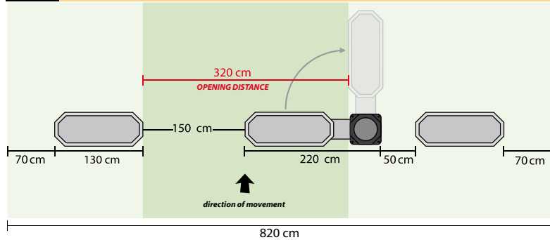
3 Mobile center and fixed sides.
