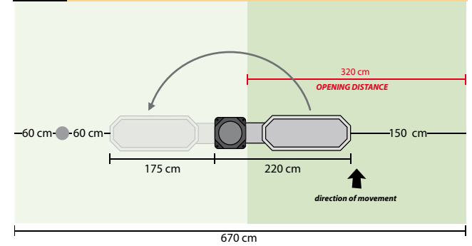
7 Barrier with 180° rotation.
