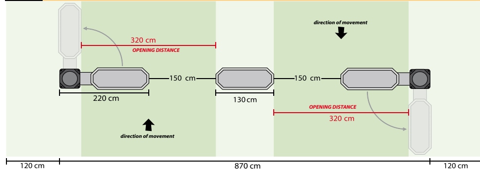
8 Fixed center + mobile sides.
