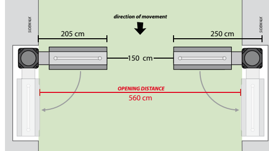
4 Double mobile with cart and built into the sidewalk.
