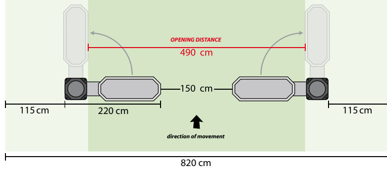
2 Double fixed side + mobile side.
