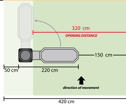
8 Fixed center + mobile sides.
