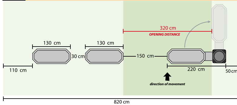
3 Mobile center and fixed sides.
